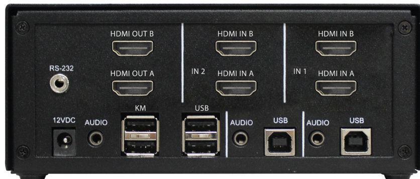
SM-UHN-2D Back
