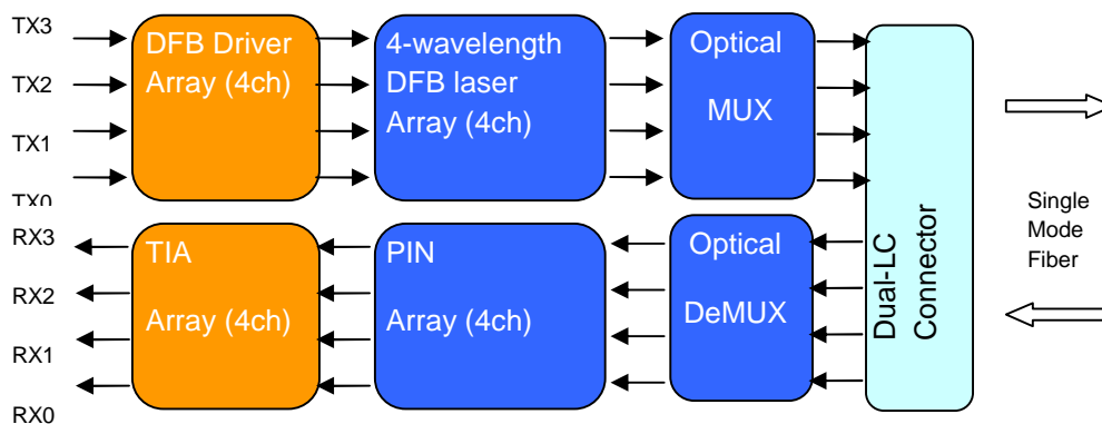
Figure 1: 40Gb/s QSFP IR4 Transceiver Block Diagram
